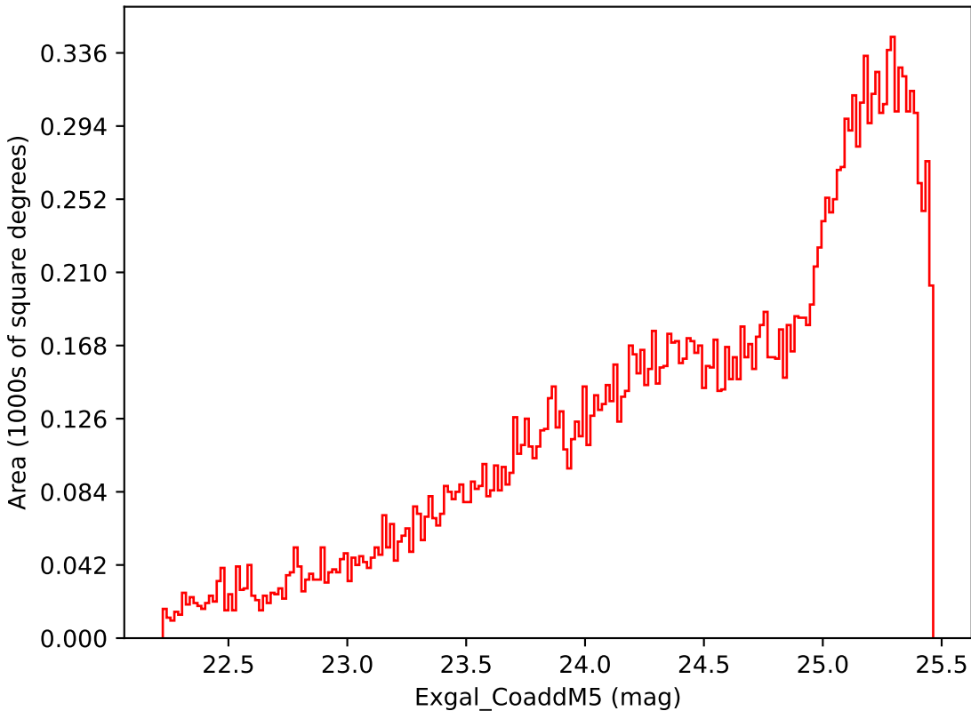
too_ignore_5_1v3.4_10yrs Yr 3-4 i band: Exgal_CoaddM5
