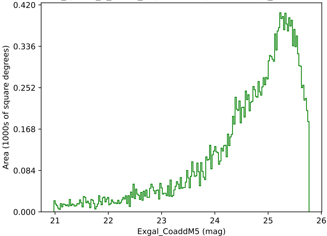
too_ignore_5_1v3.4_10yrs Yr 3-4 g band: Exgal_CoaddM5
