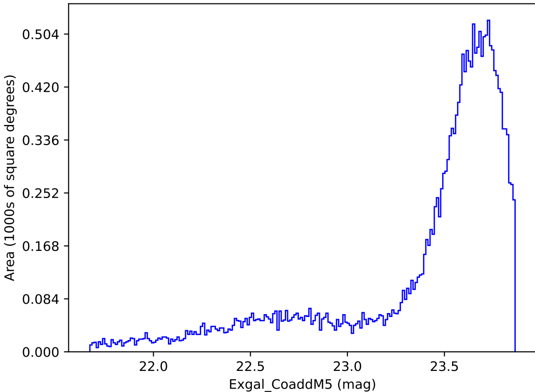
too_ignore_5_1v3.4_10yrs Yr 1 y band: Exgal_CoaddM5
