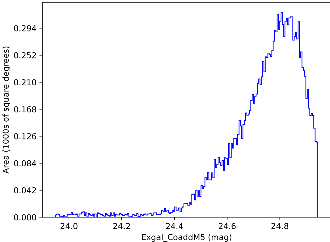
too_ignore_5_1v3.4_10yrs WFD y band: Exgal_CoaddM5
