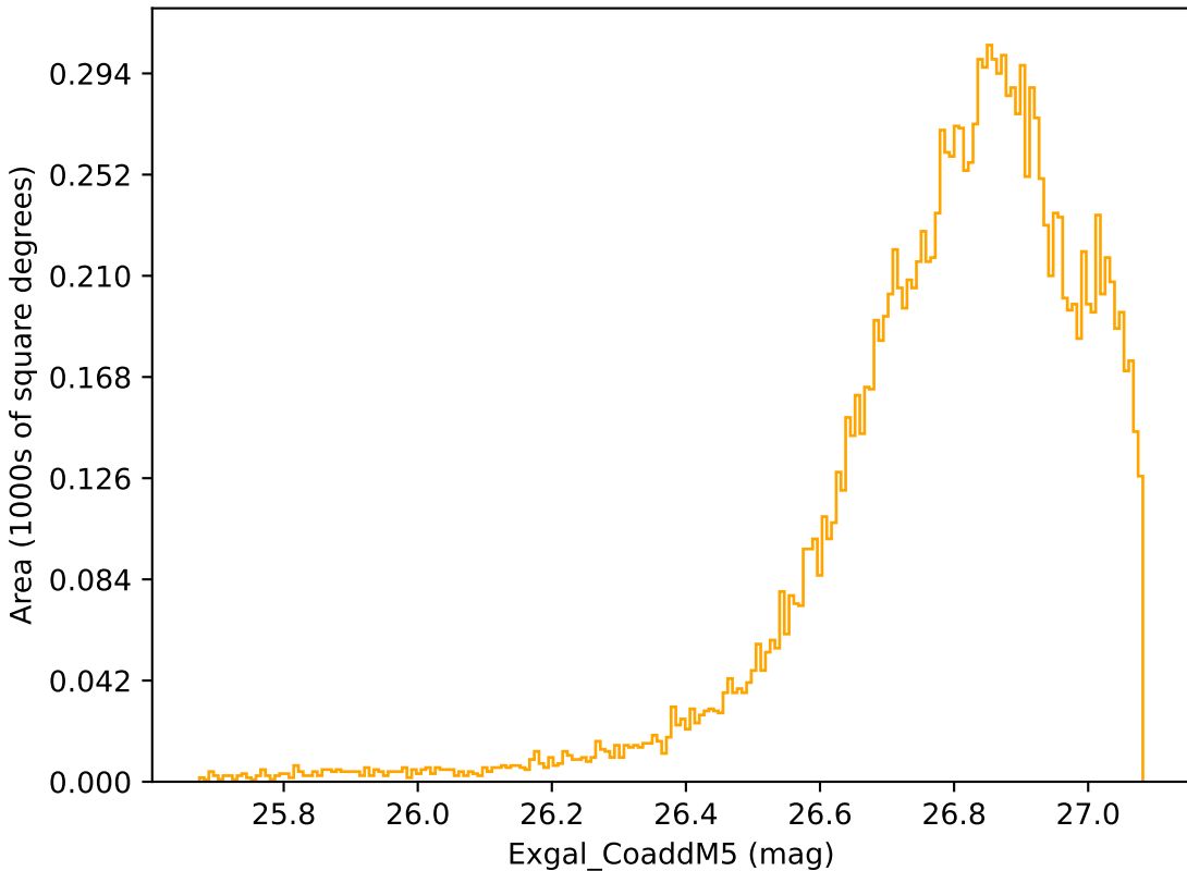
too_ignore_5_1v3.4_10yrs WFD r band: Exgal_CoaddM5
