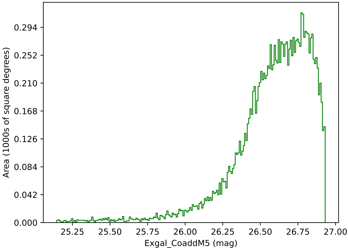
too_ignore_5_1v3.4_10yrs WFD g band: Exgal_CoaddM5
