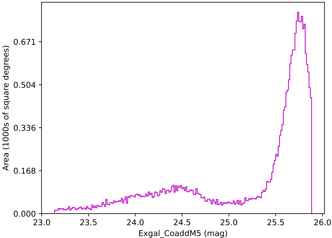
too_ignore_5_1v3.4_10yrs All sky z band: Exgal_CoaddM5
