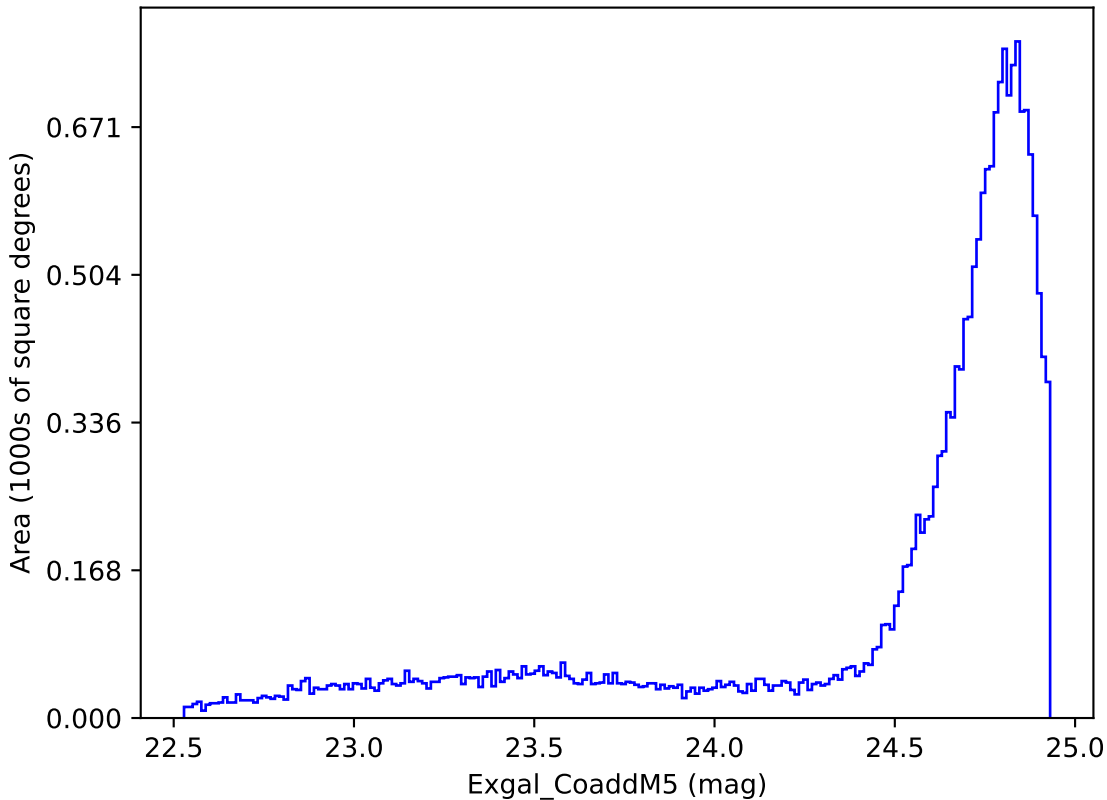
too_ignore_5_1v3.4_10yrs All sky y band: Exgal_CoaddM5
