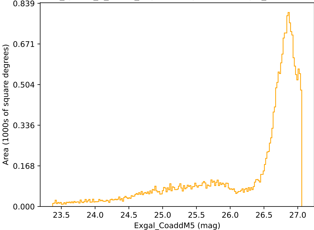
too_ignore_5_1v3.4_10yrs All sky r band: Exgal_CoaddM5
