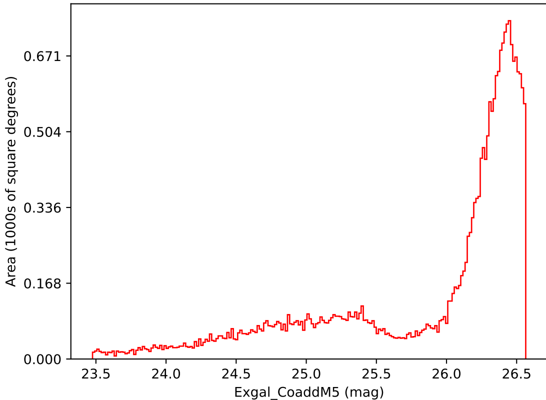
too_ignore_5_1v3.4_10yrs All sky i band: Exgal_CoaddM5
