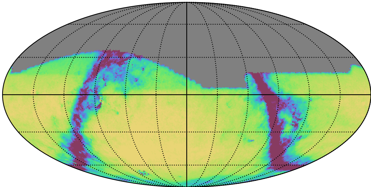
too_ignore_5_1v3.4_10yrs All sky g band: Exgal_CoaddM5
