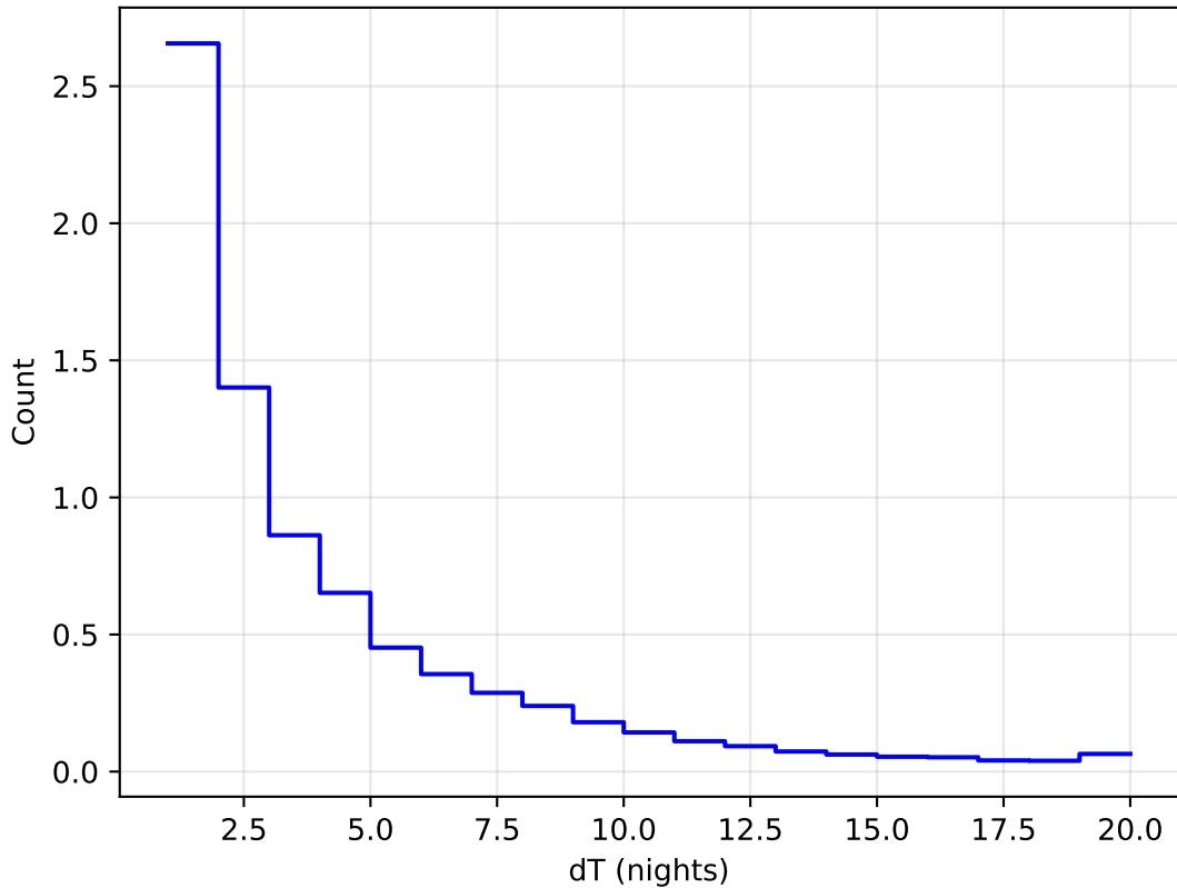
too_ignore_5_1v3.4_10yrs WFD all bands: DeltaNight Histogram 1e6
