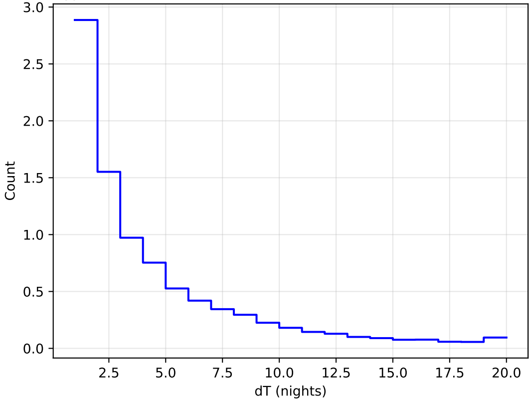
too_ignore_5_1v3.4_10yrs All sky all bands: DeltaNight Histogram 1e6
