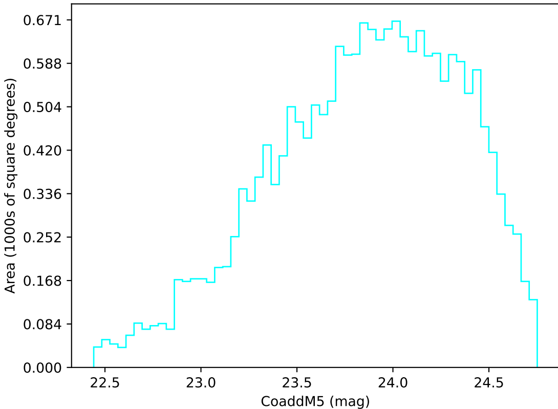
too_ignore_5_1v3.4_10yrs Yr 3-4 u band: CoaddM5
