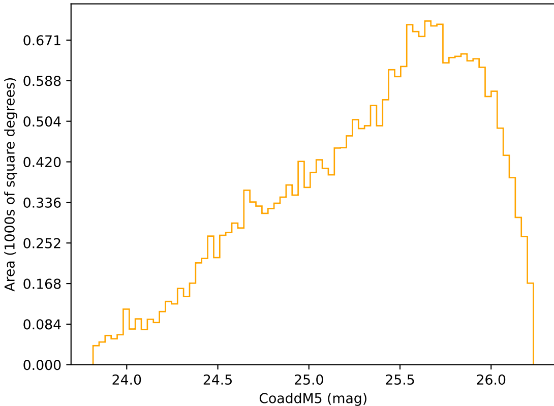
too_ignore_5_1v3.4_10yrs Yr 3-4 r band: CoaddM5
