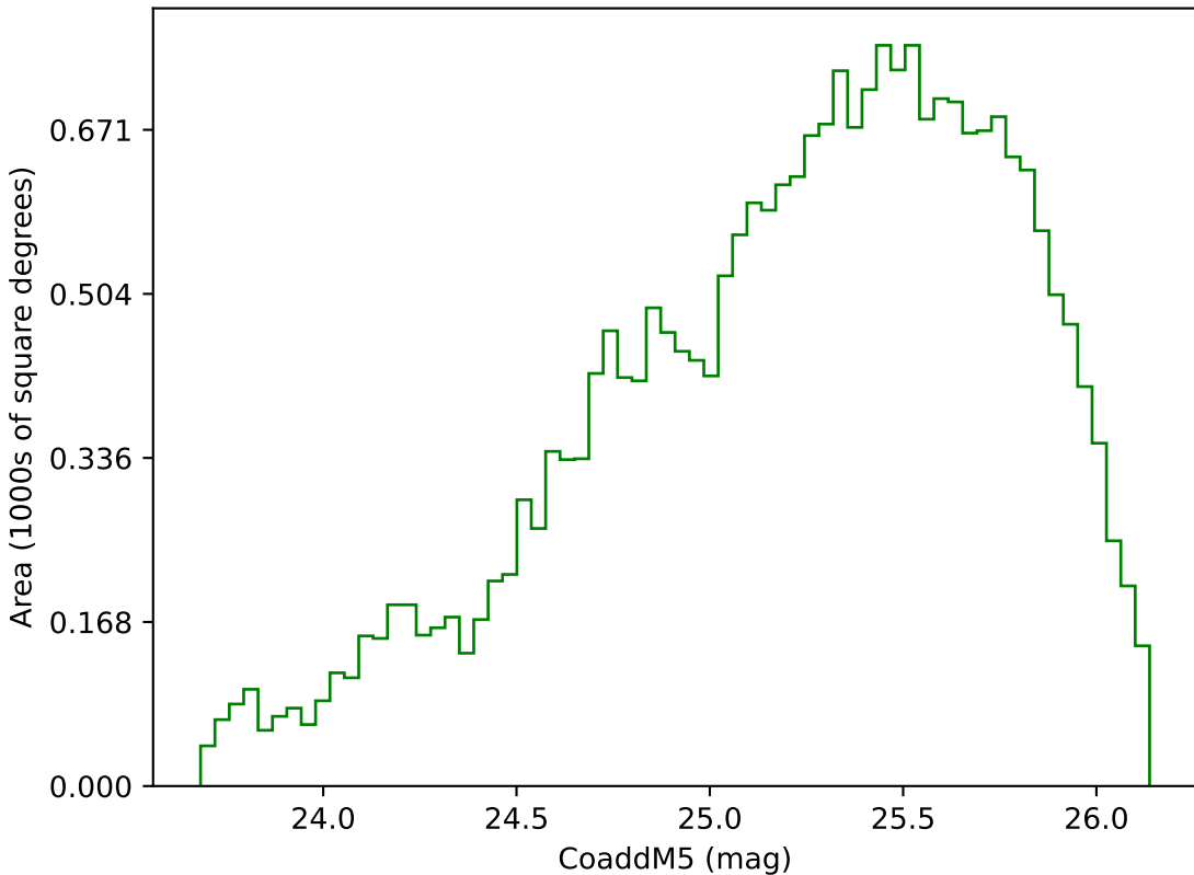
too_ignore_5_1v3.4_10yrs Yr 3-4 g band: CoaddM5
