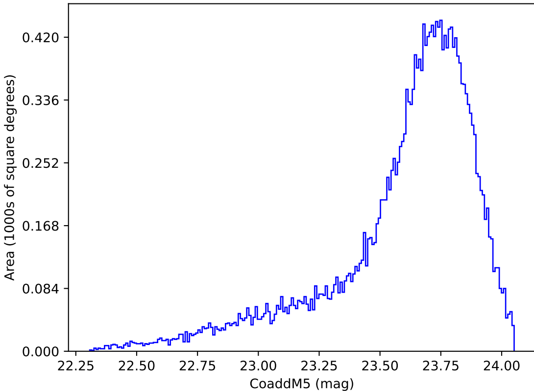
too_ignore_5_1v3.4_10yrs Yr 1 y band: CoaddM5
