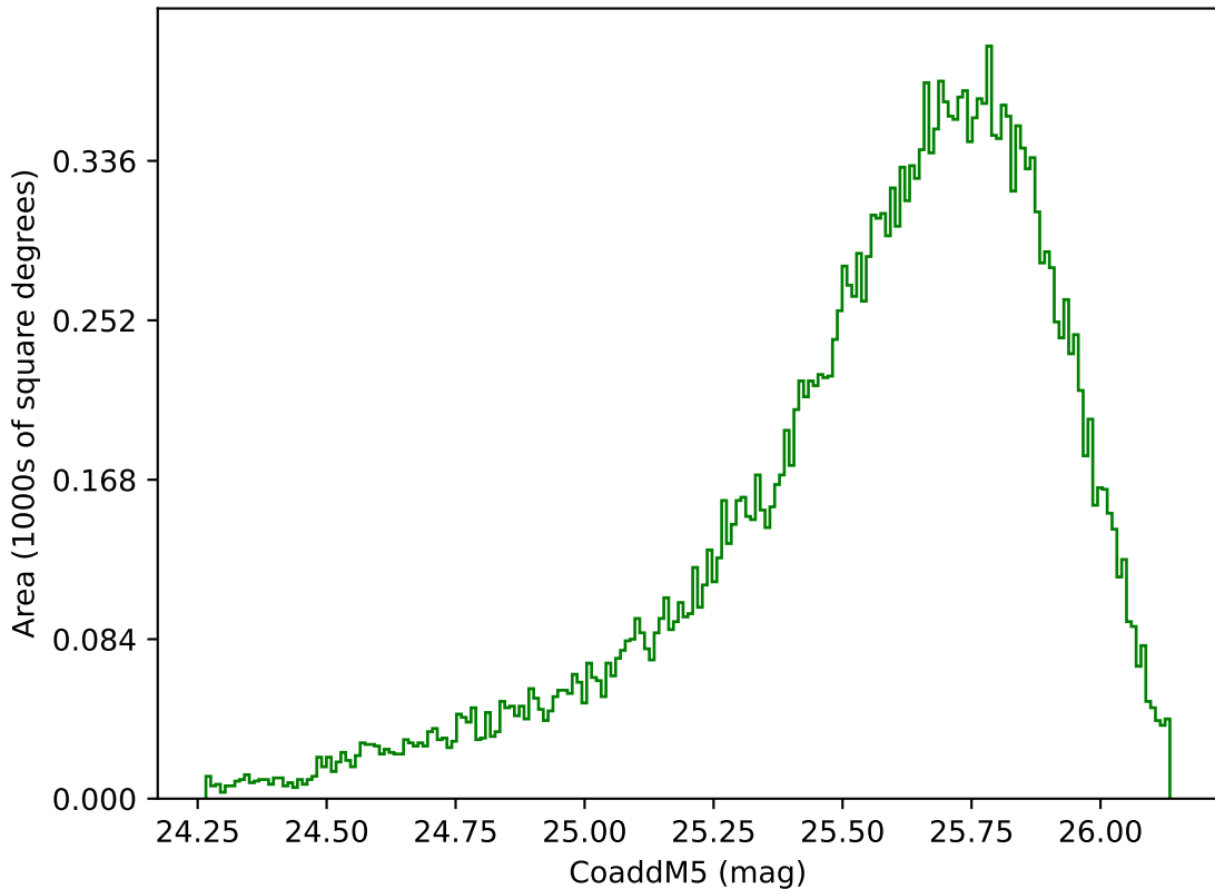
too_ignore_5_1v3.4_10yrs Yr 1 g band: CoaddM5
