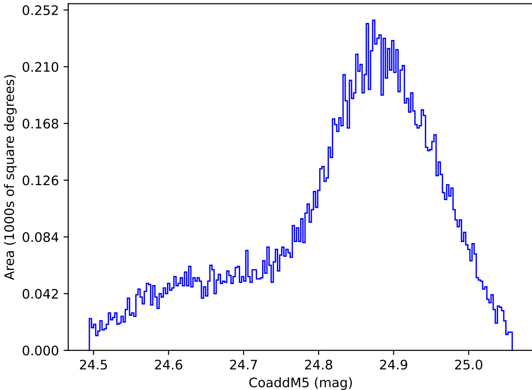
too_ignore_5_1v3.4_10yrs WFD y band: CoaddM5
