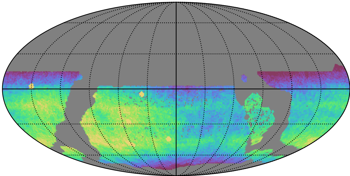
too_ignore_5_1v3.4_10yrs WFD r band: CoaddM5
