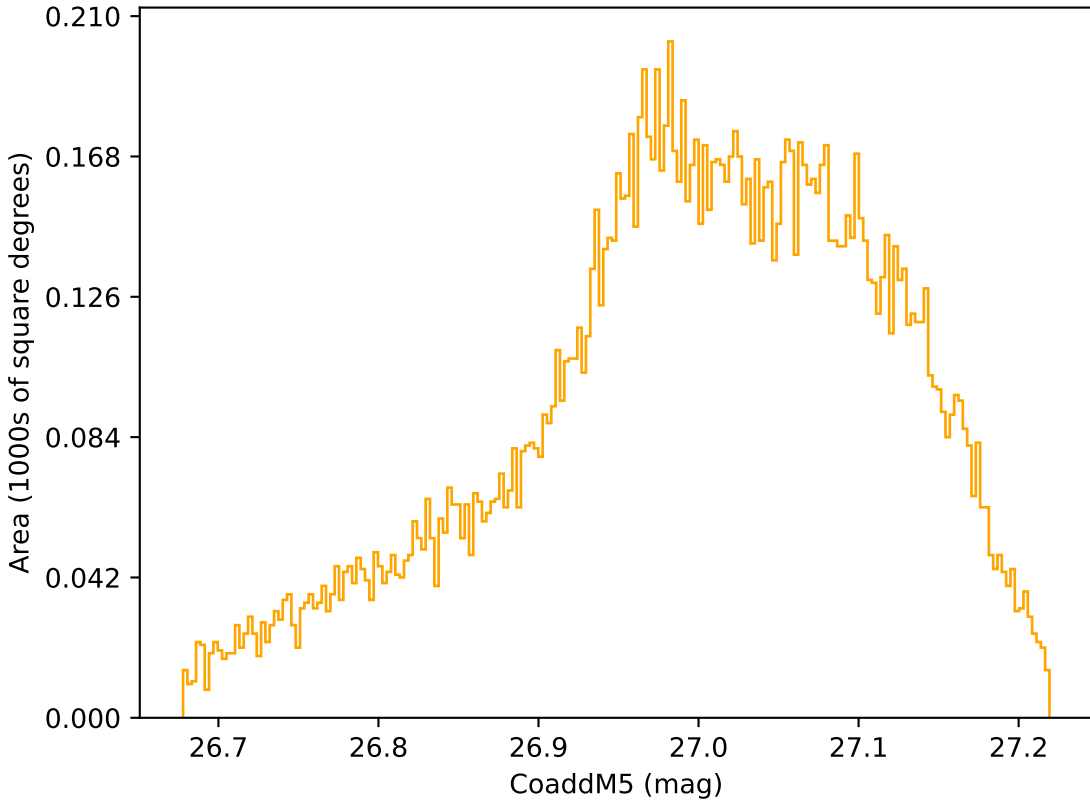
too_ignore_5_1v3.4_10yrs WFD r band: CoaddM5
