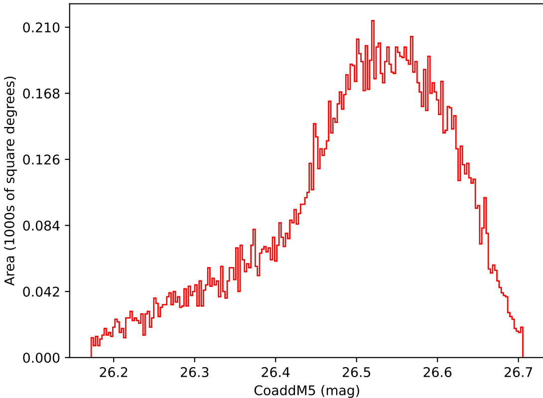
too_ignore_5_1v3.4_10yrs WFD i band: CoaddM5
