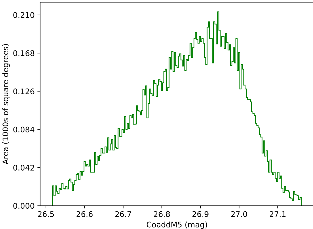
too_ignore_5_1v3.4_10yrs WFD g band: CoaddM5
