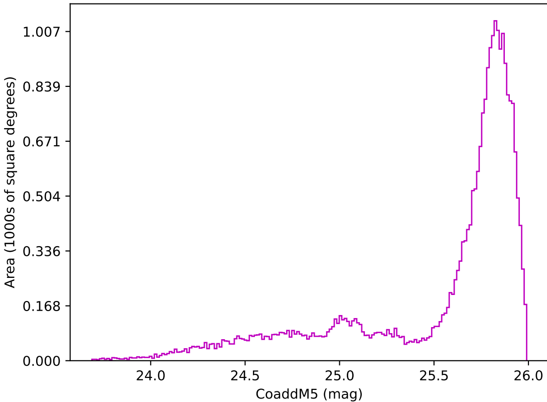
too_ignore_5_1v3.4_10yrs All sky z band: CoaddM5
