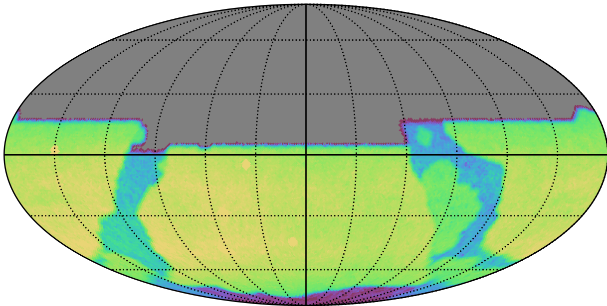
too_ignore_5_1v3.4_10yrs All sky y band: CoaddM5
