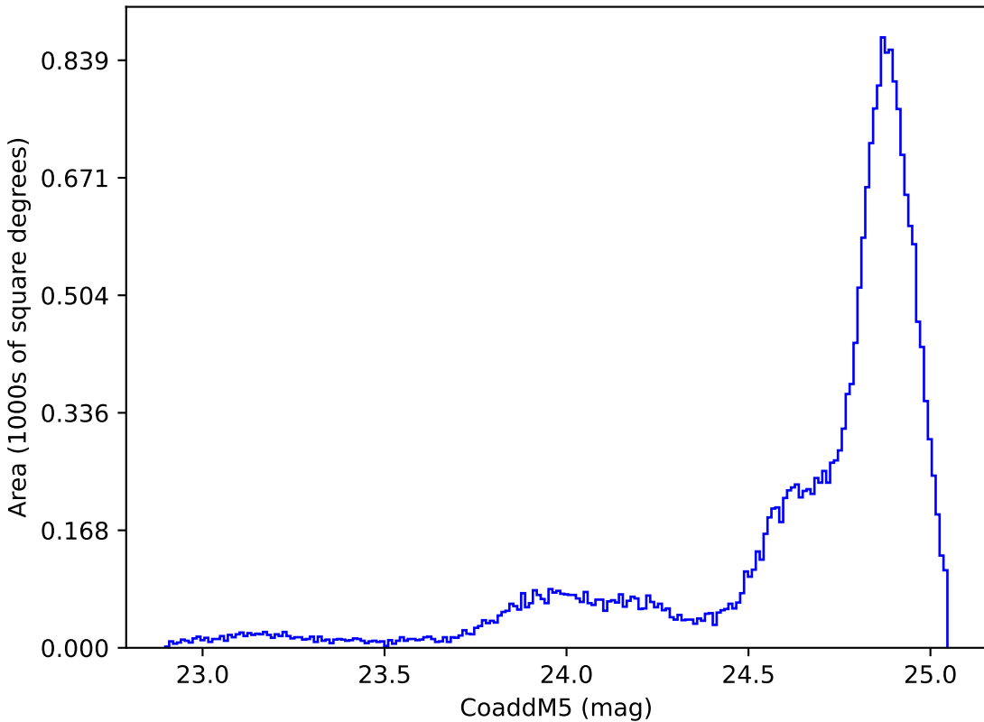
too_ignore_5_1v3.4_10yrs All sky y band: CoaddM5
