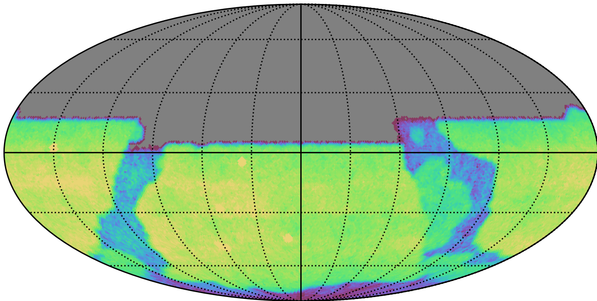
too_ignore_5_1v3.4_10yrs All sky u band: CoaddM5
