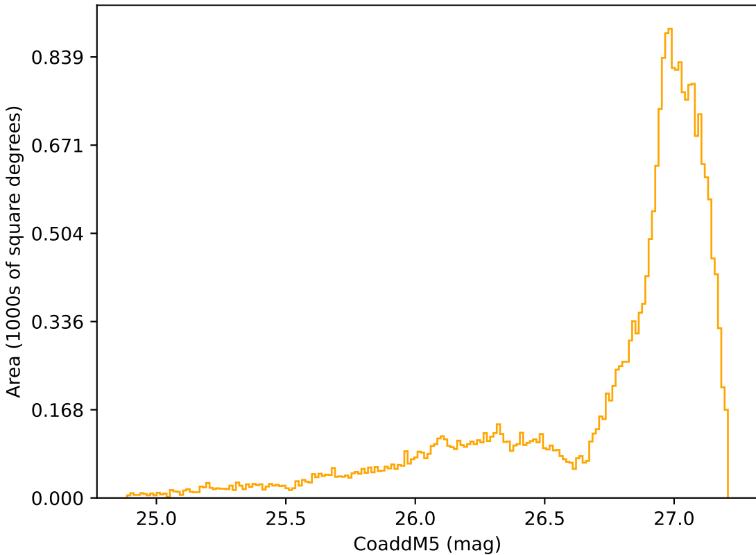
too_ignore_5_1v3.4_10yrs All sky r band: CoaddM5
