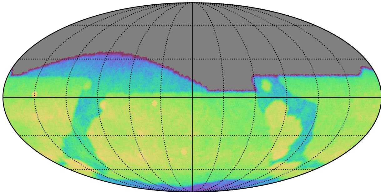
too_ignore_5_1v3.4_10yrs All sky g band: CoaddM5
