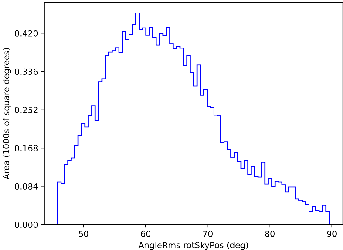
too_ignore_5_1v3.4_10yrs WFD y band: AngleRms rotSkyPos
