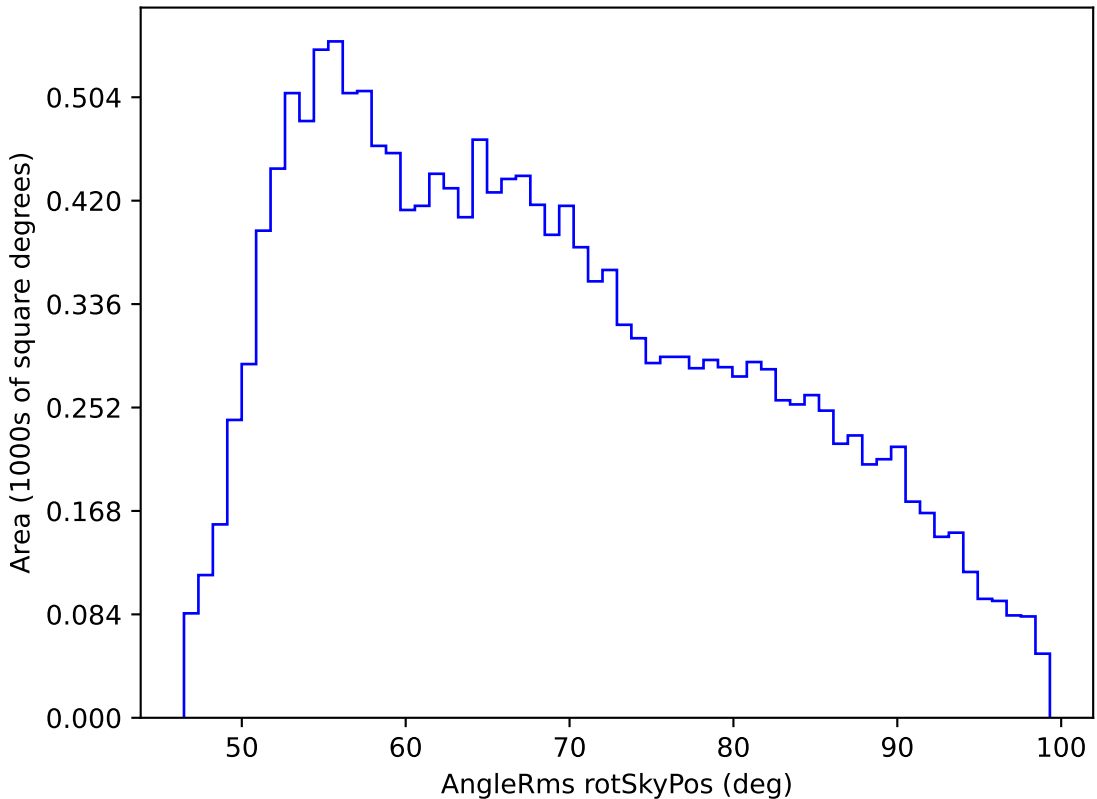
too_ignore_5_1v3.4_10yrs WFD g band: AngleRms rotSkyPos
