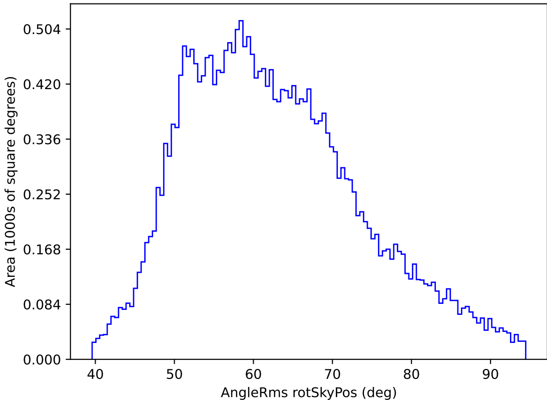
too_ignore_5_1v3.4_10yrs All sky z band: AngleRms rotSkyPos
