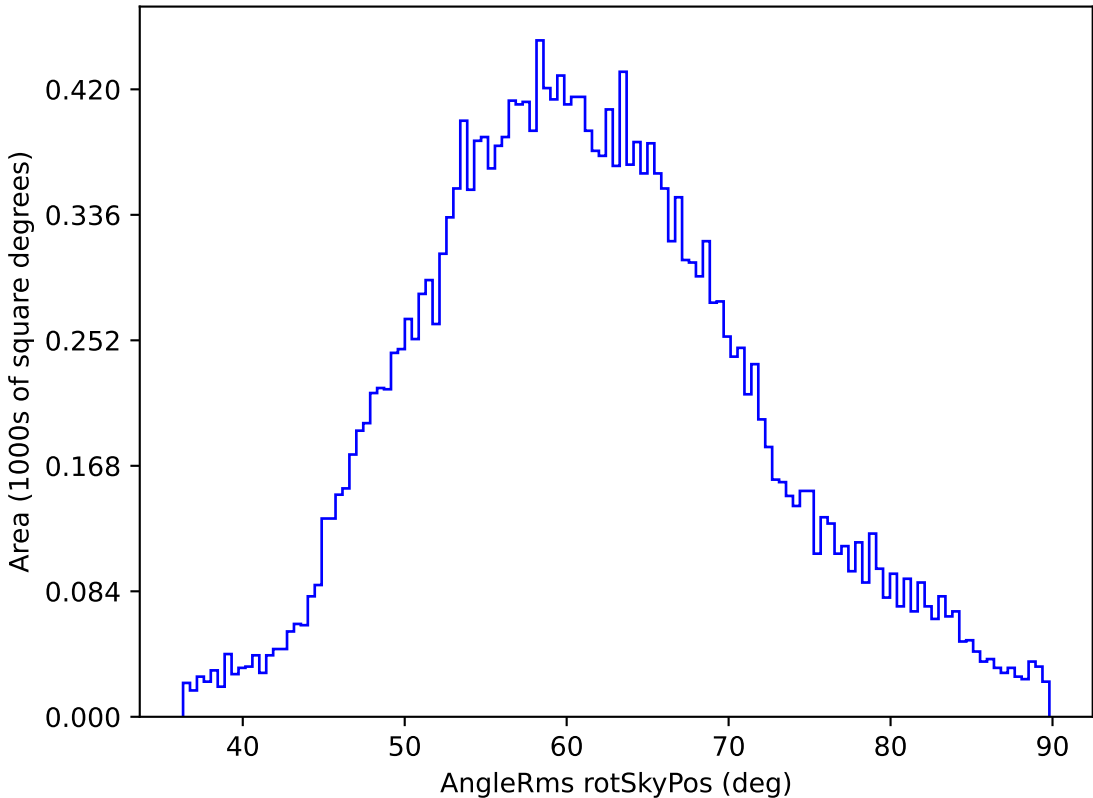
too_ignore_5_1v3.4_10yrs All sky y band: AngleRms rotSkyPos
