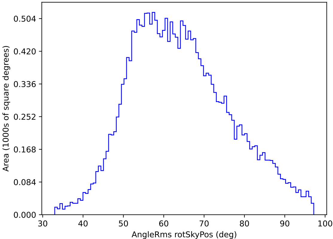
too_ignore_5_1v3.4_10yrs All sky u band: AngleRms rotSkyPos
