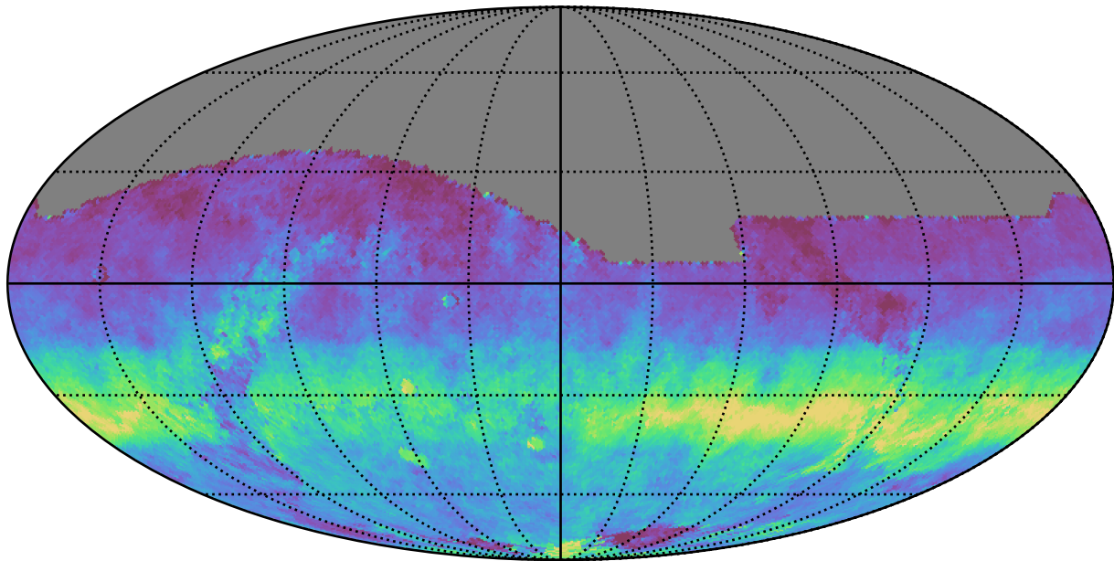
too_ignore_5_1v3.4_10yrs All sky r band: AngleRms rotSkyPos
