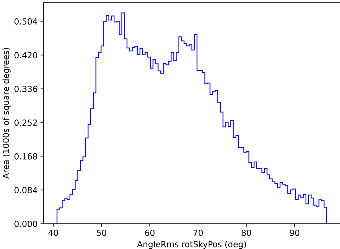
too_ignore_5_1v3.4_10yrs All sky r band: AngleRms rotSkyPos
