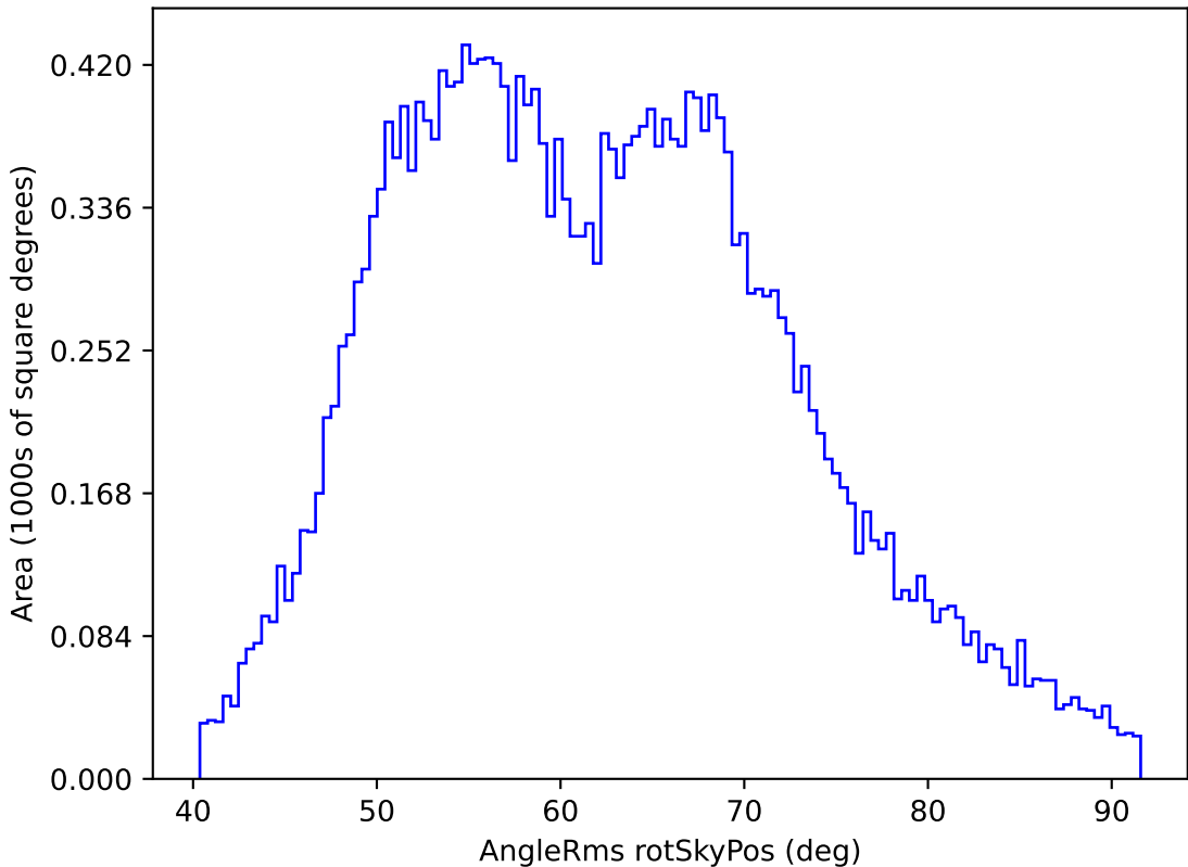
too_ignore_5_1v3.4_10yrs All sky i band: AngleRms rotSkyPos
