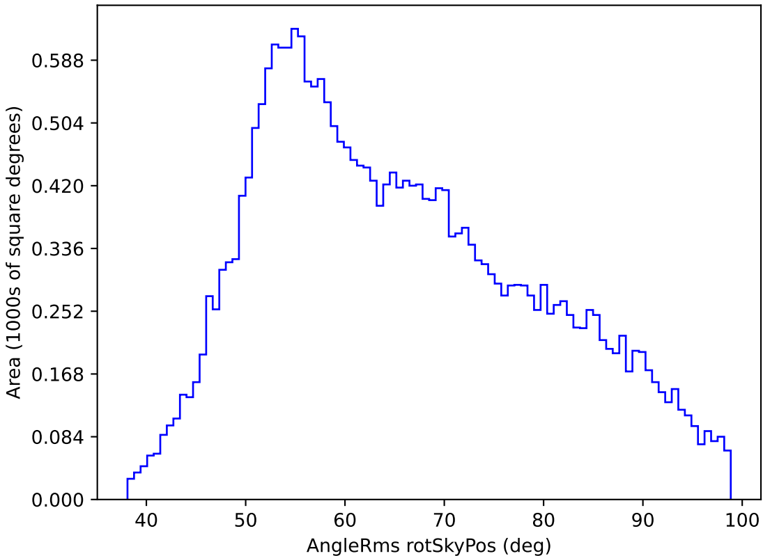
too_ignore_5_1v3.4_10yrs All sky g band: AngleRms rotSkyPos
