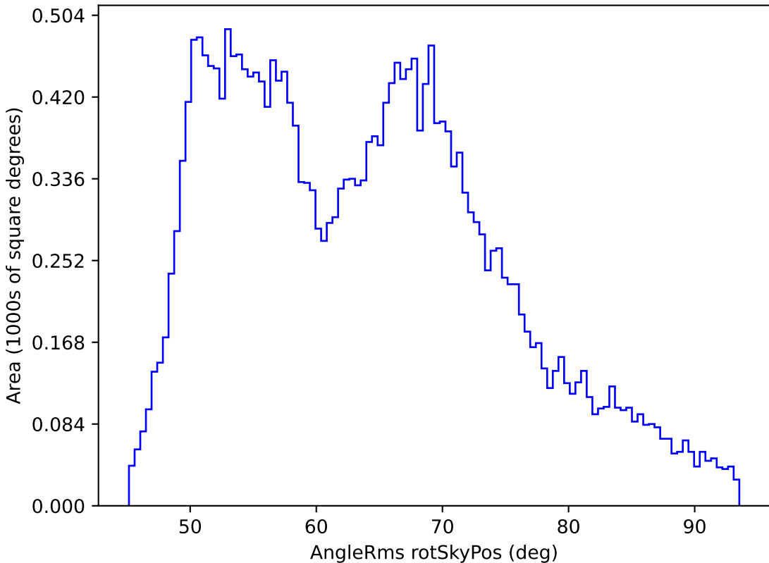
too_ignore_5_1v3.4_10yrs All sky all bands: AngleRms rotSkyPos
