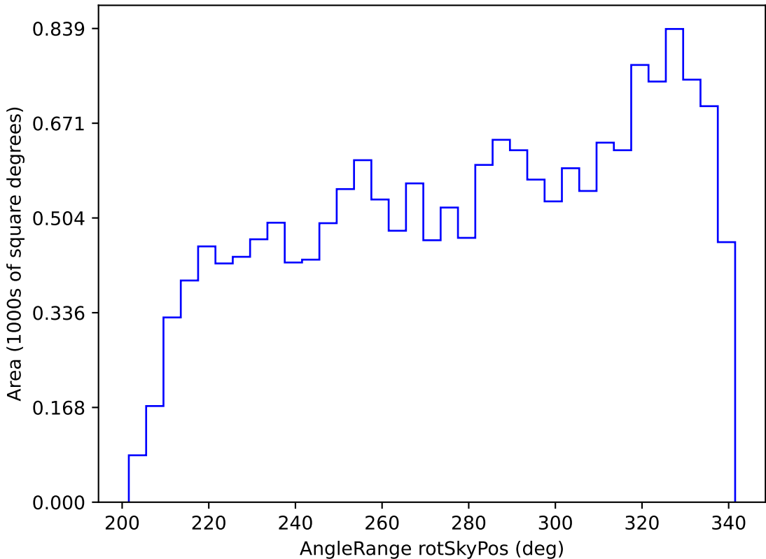
too_ignore_5_1v3.4_10yrs WFD z band: AngleRange rotSkyPos
