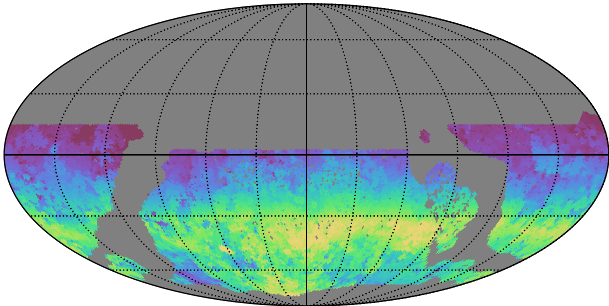
too_ignore_5_1v3.4_10yrs WFD y band: AngleRange rotSkyPos
