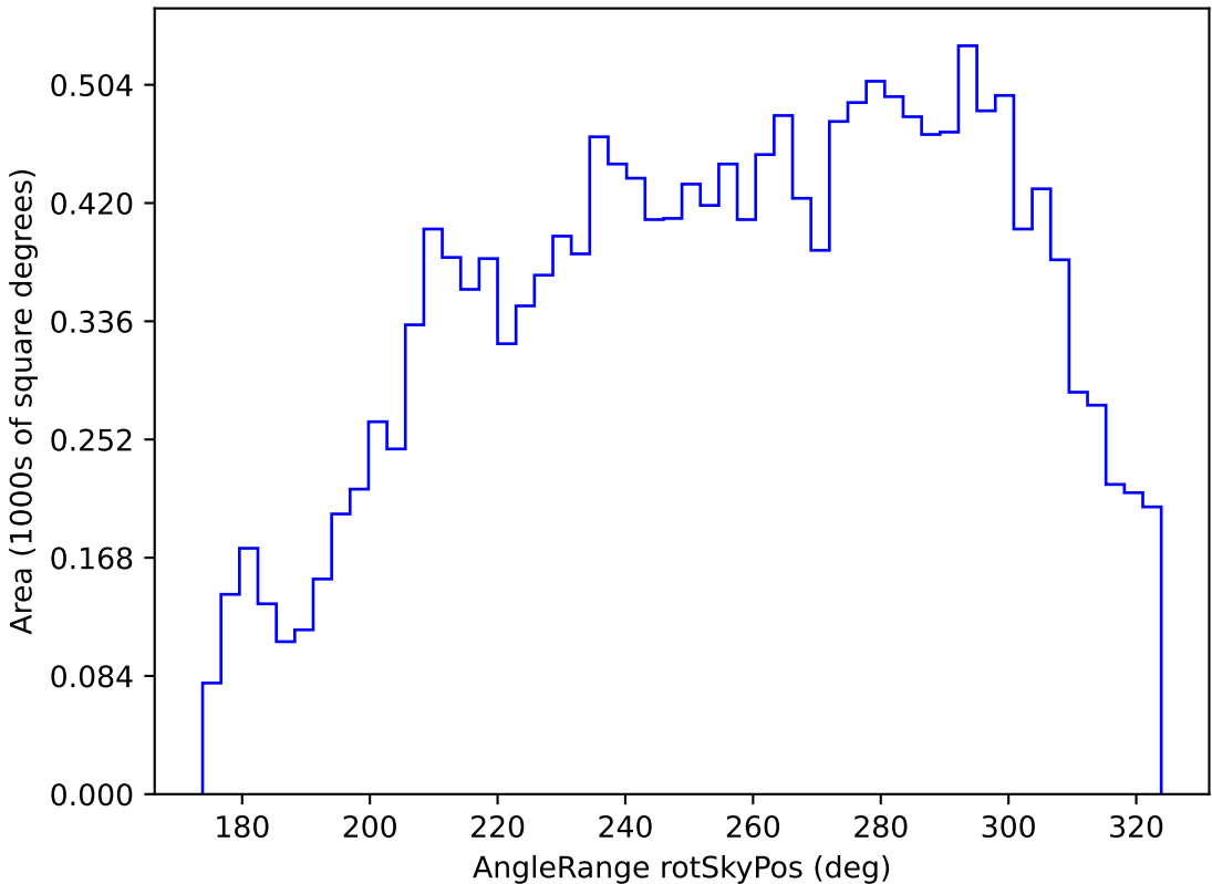
too_ignore_5_1v3.4_10yrs WFD u band: AngleRange rotSkyPos
