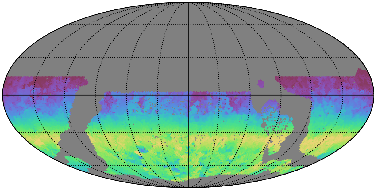
too_ignore_5_1v3.4_10yrs WFD r band: AngleRange rotSkyPos
