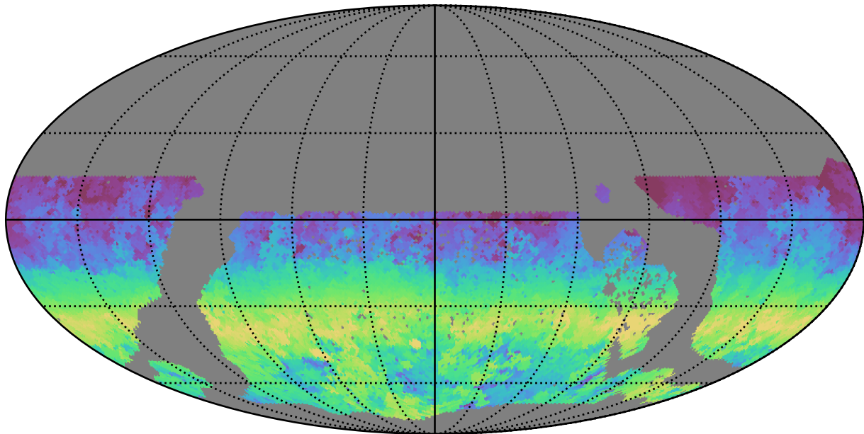
too_ignore_5_1v3.4_10yrs WFD g band: AngleRange rotSkyPos
