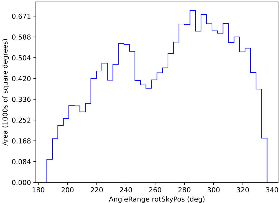
too_ignore_5_1v3.4_10yrs WFD g band: AngleRange rotSkyPos
