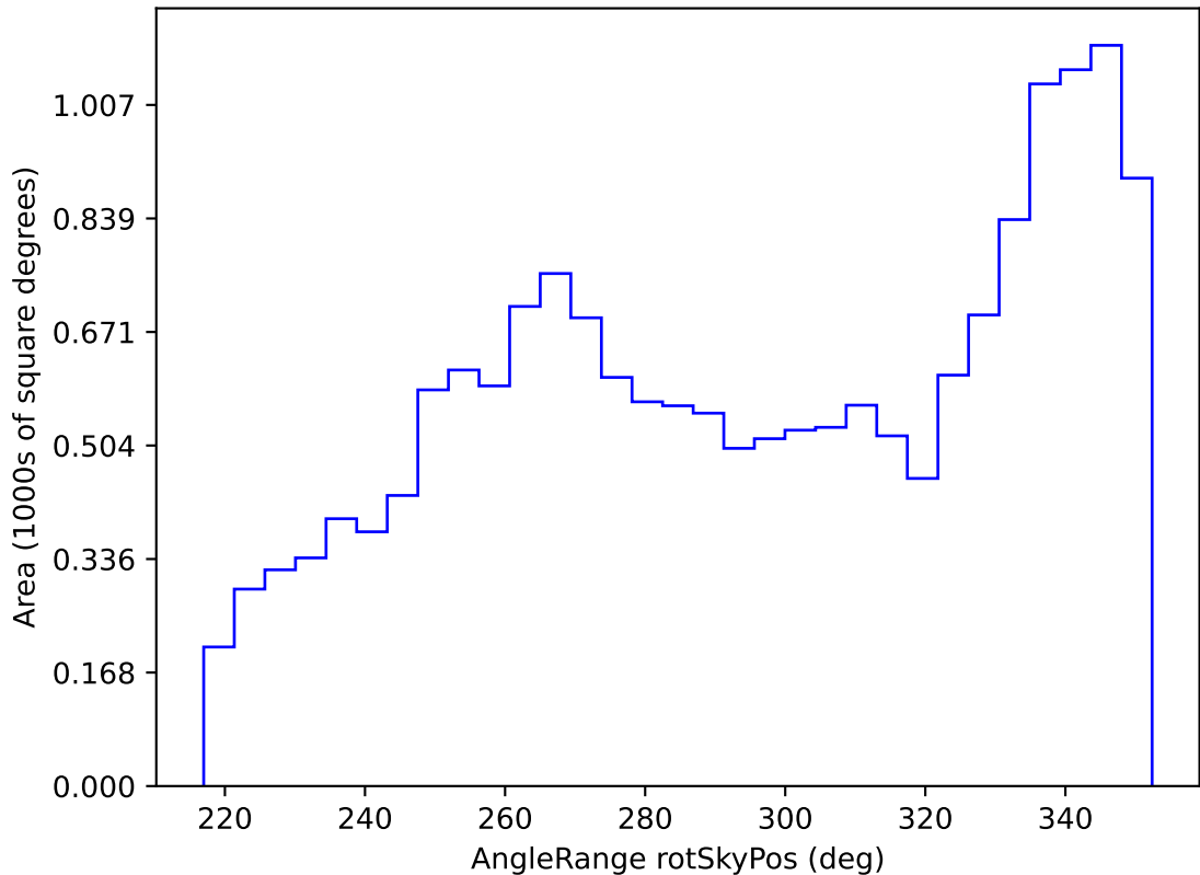
too_ignore_5_1v3.4_10yrs WFD all bands: AngleRange rotSkyPos
