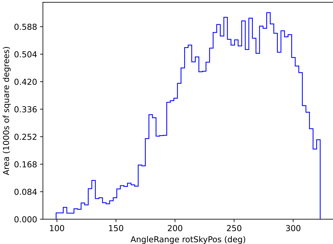
too_ignore_5_1v3.4_10yrs All sky u band: AngleRange rotSkyPos
