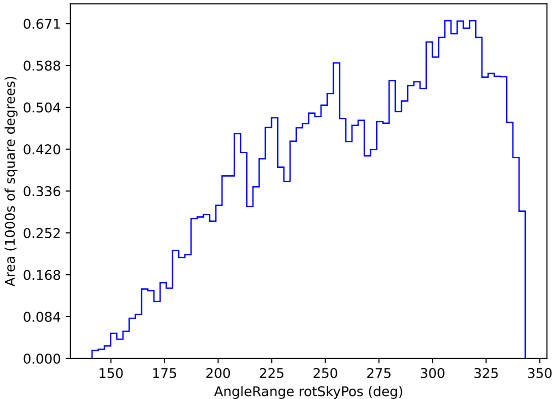
too_ignore_5_1v3.4_10yrs All sky r band: AngleRange rotSkyPos
