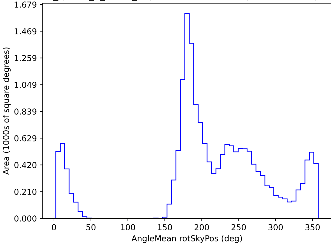
too_ignore_5_1v3.4_10yrs WFD z band: AngleMean rotSkyPos
