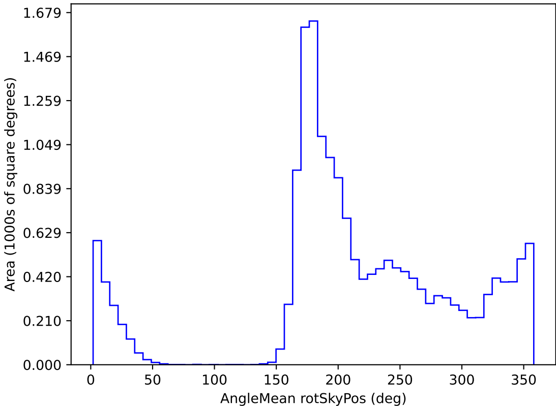
too_ignore_5_1v3.4_10yrs WFD u band: AngleMean rotSkyPos
